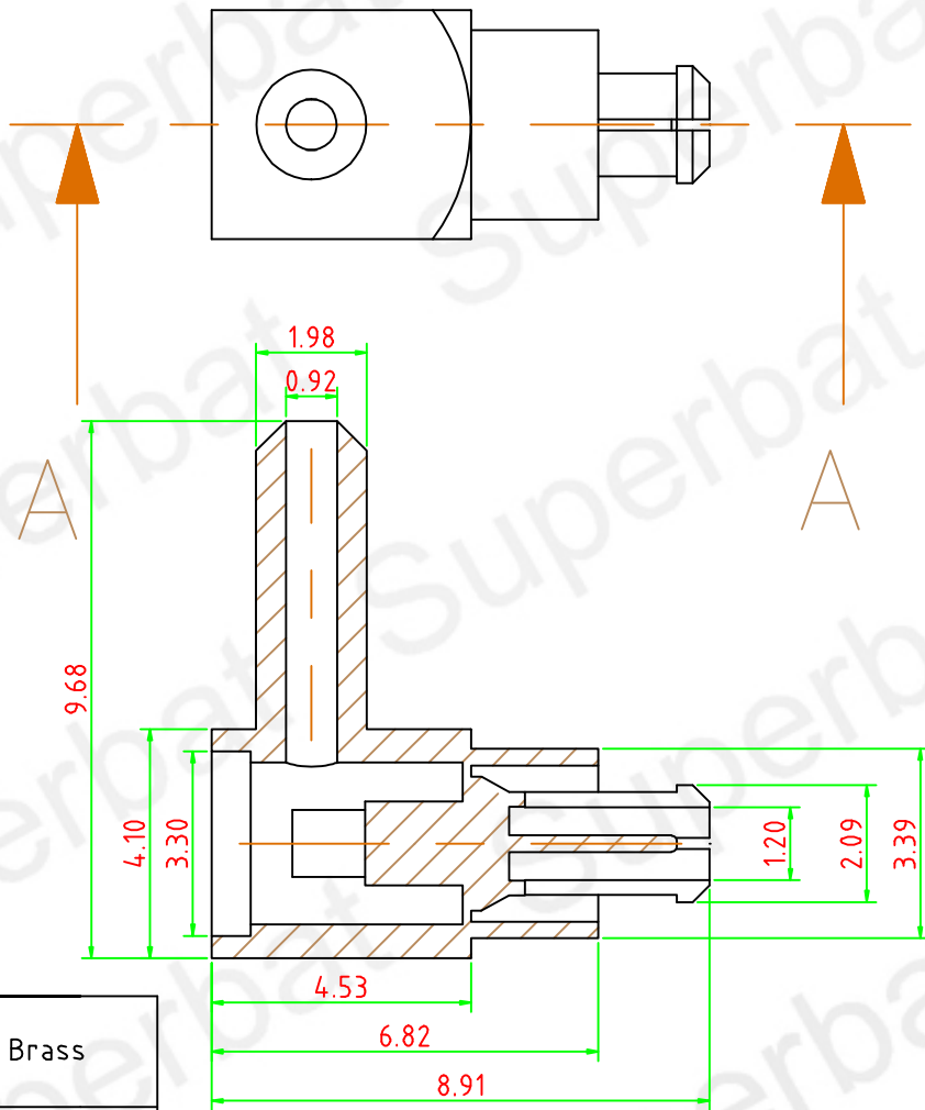
SECTION A—A
